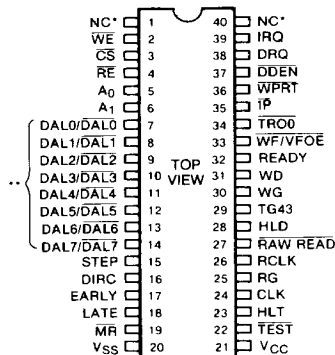
PACKAGE DIP-40C-A01
