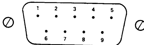
PADDLE PORT CONNECTOR (9 PIN D)
