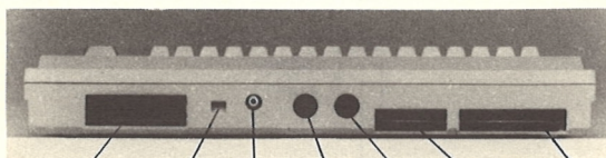
④ ⑤ ⑥ ⑦ ⑧ ⑨ ⑩ CARTRIDGE CHANNEL TV AUDIO/VIDEO SERIAL CASSETTE USER SLOT SELECTOR CONNECTOR CONNECTOR PORT INTERFACE PORT
