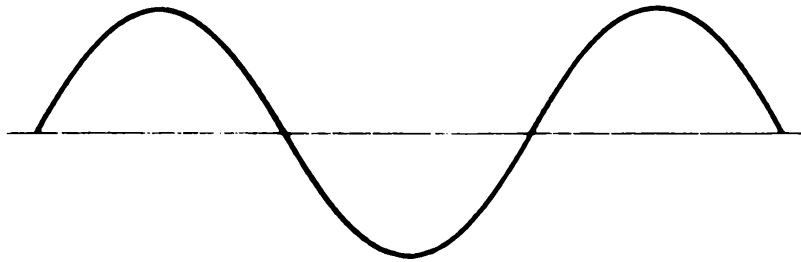
Figure 7-1. Sine Wave
