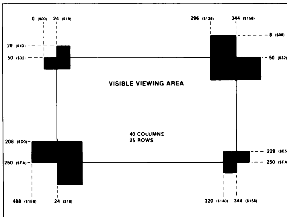
Figure 6-7. Visible Sprite Coordinates
