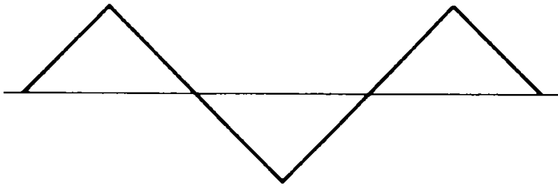
TRIANGLE
