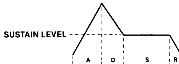
Figure 7-4. ADSR Phases
