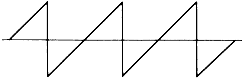
SAWTOOTH
