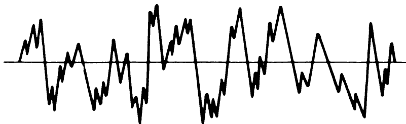
NOISE
