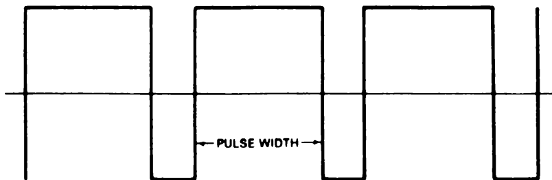
VARIABLE PULSE
