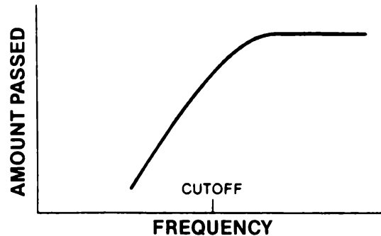
Figure 7-8. High-pass Filter
